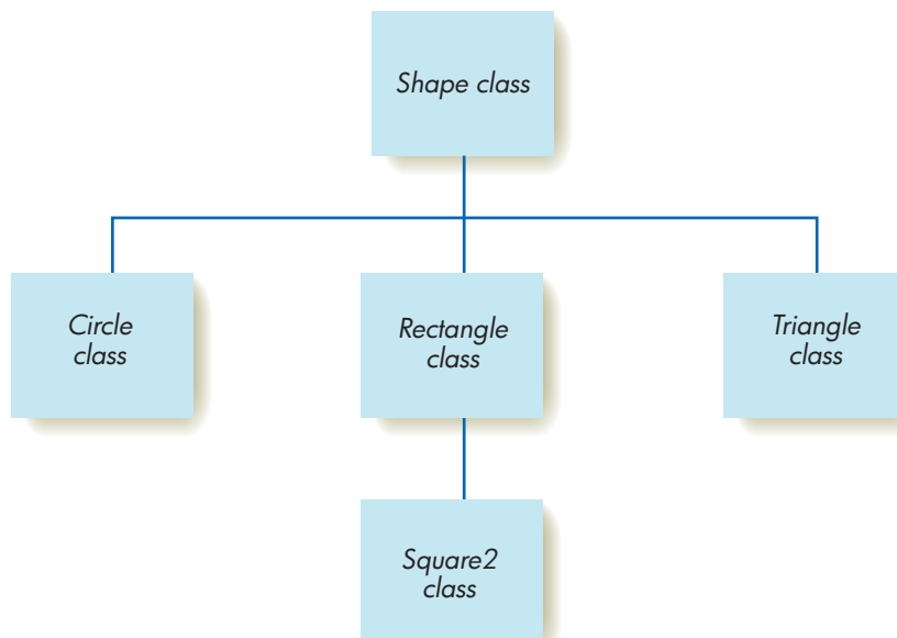
FIGURE 31 A Hierarchy of Geometric Classes
